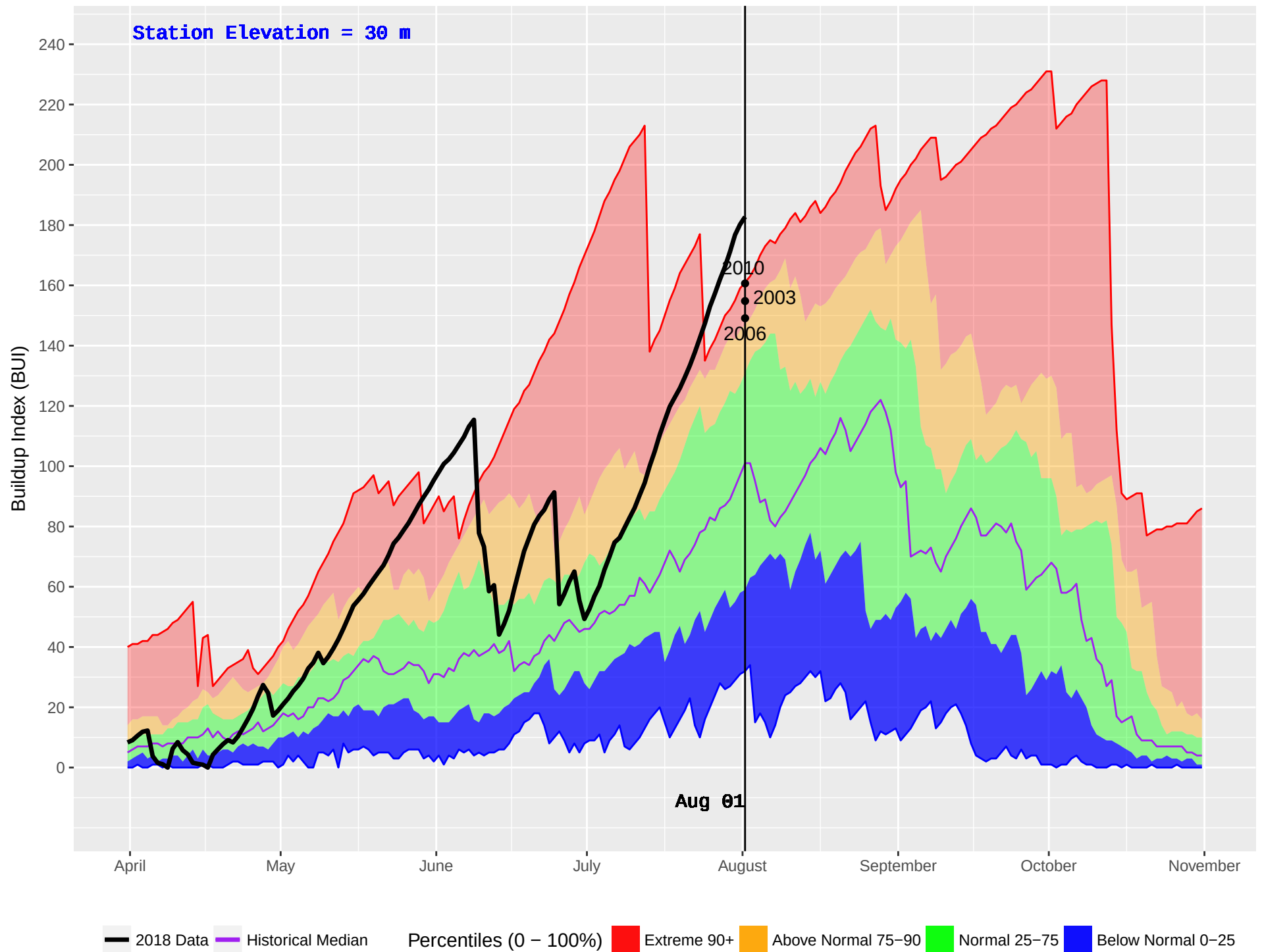
CEDAR (59) : Historical (1989–2016) and Current (2018) Daily Buildup Index (BUI)
