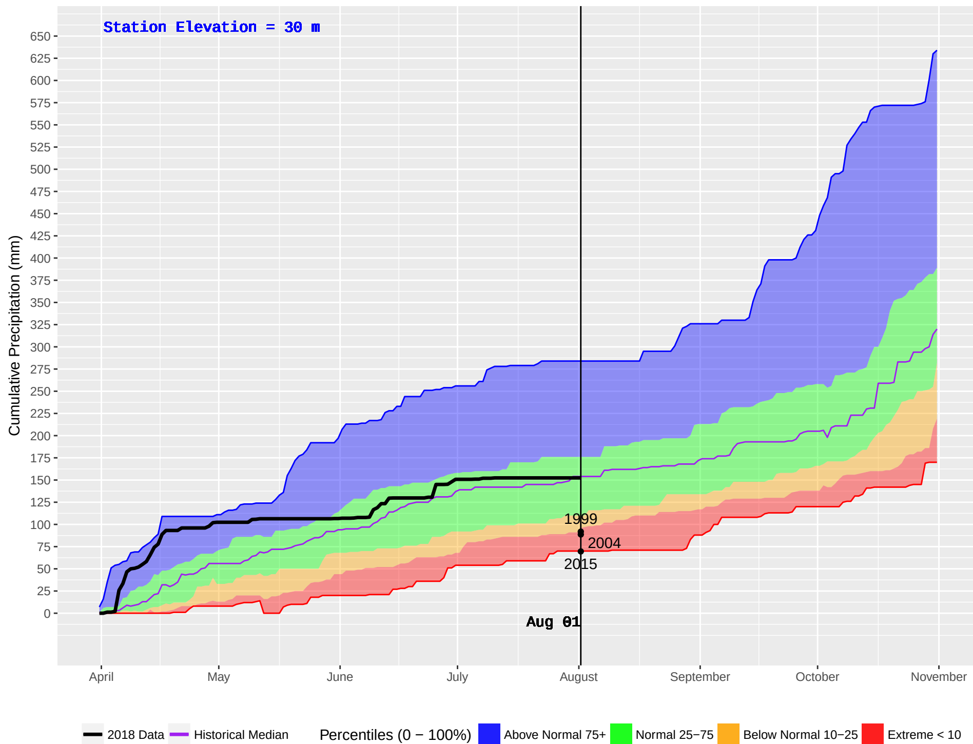
CEDAR (59) : Historical (1989–2016) and Current (2018) Daily Cumulative Precipitation
