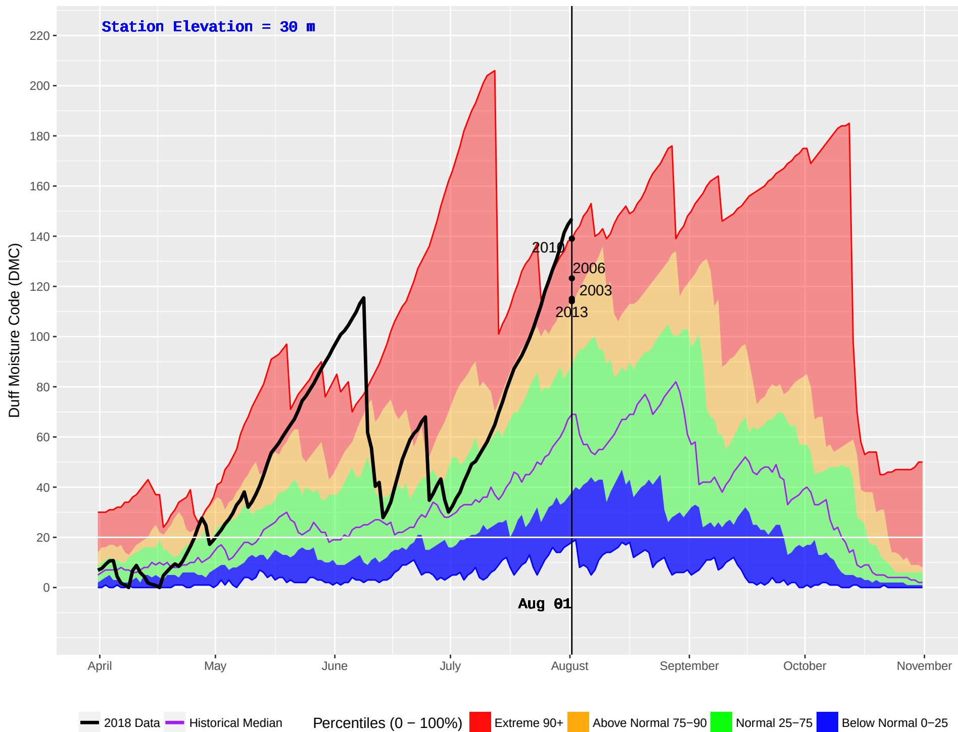
CEDAR (59) : Historical (1989–2016) and Current (2018) Daily Duff Moisture Code (DMC)
