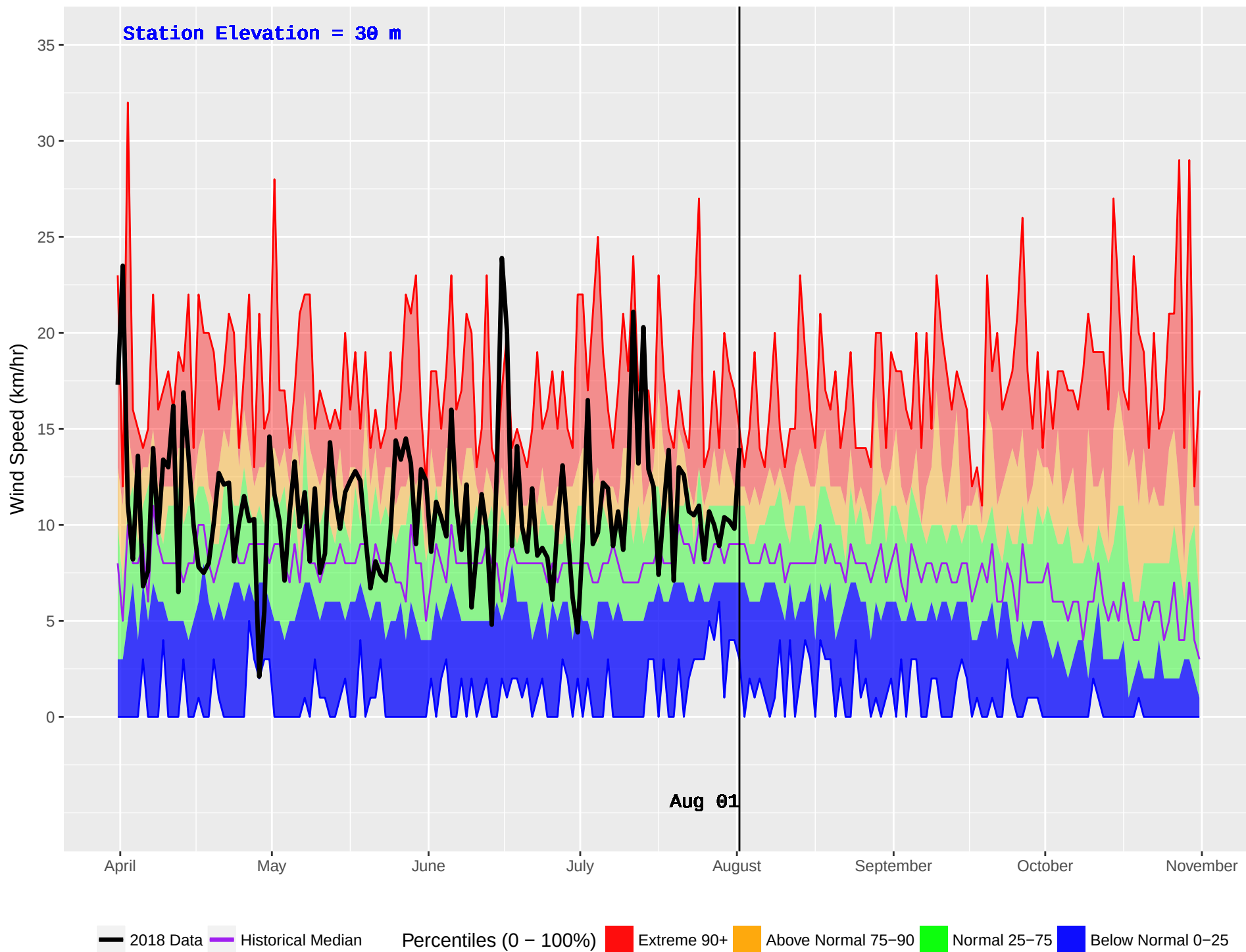
CEDAR (59) : Historical (1989–2016) and Current (2018) Daily Wind Speed
