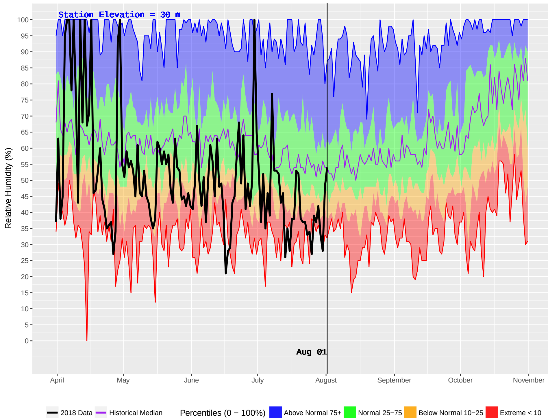
CEDAR (59) : Historical (1989–2016) and Current (2018) Daily Relative Humidity
