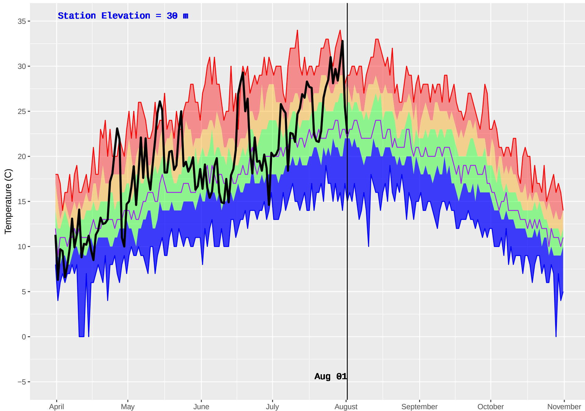
CEDAR (59) : Historical (1989–2016) and Current (2018) Daily Temperature
